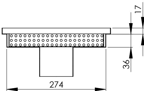
Cross-section A-A
