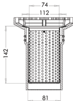
Cross Section
