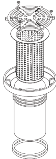
FW-150R-BASKET
